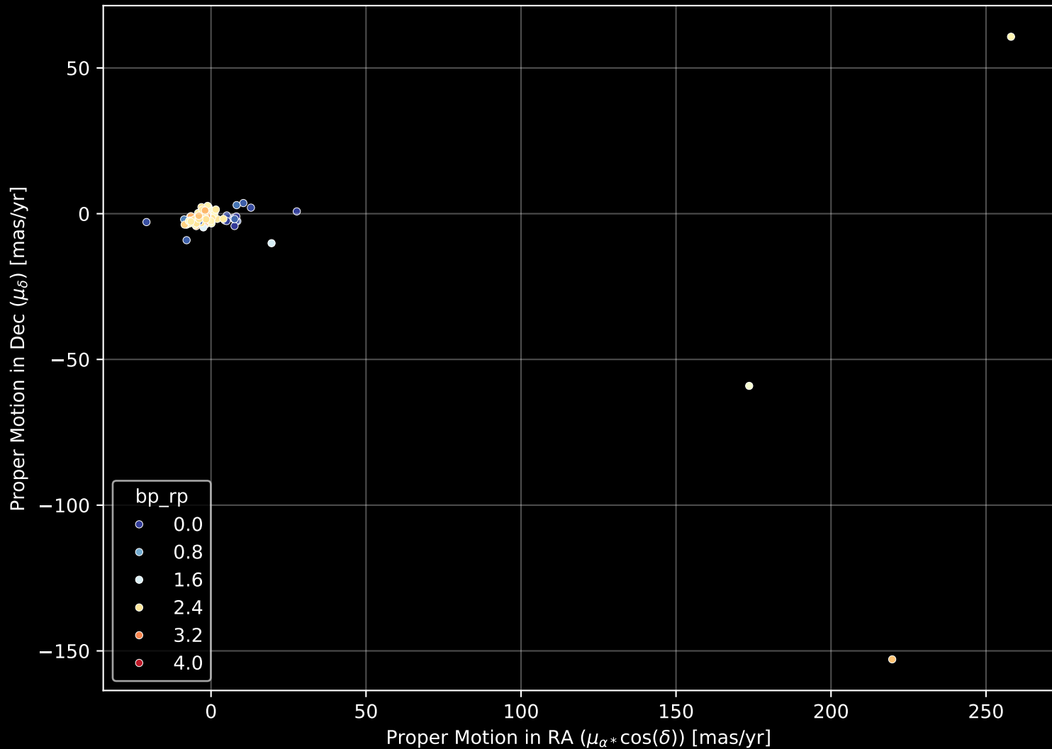
APOGEE DR17 Field: [113+04] Proper Motion Diagram (n= 156)
