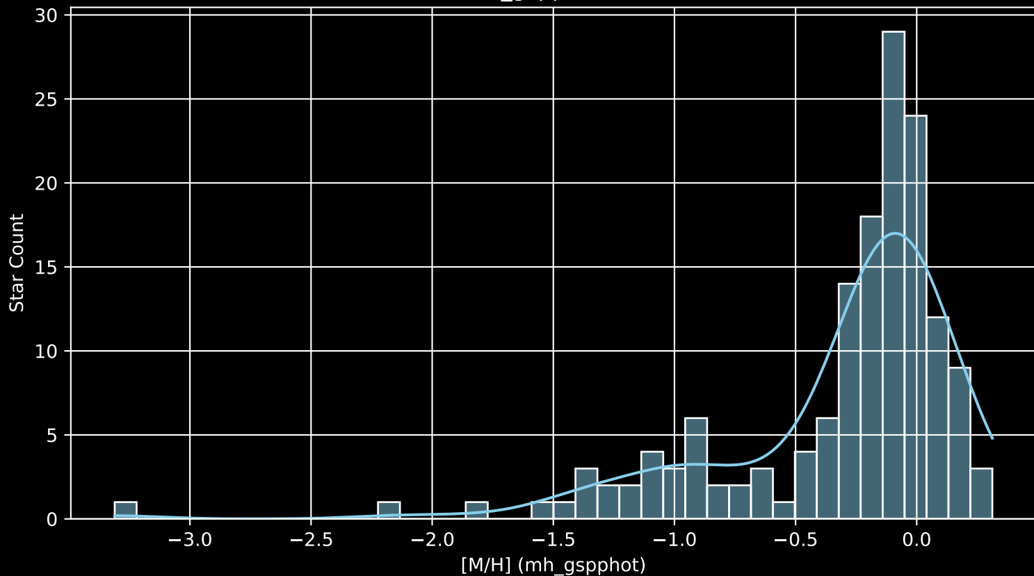
APOGEE DR17 Field: [113+04 [M/H] (mh_gspphot) (n= 152)
