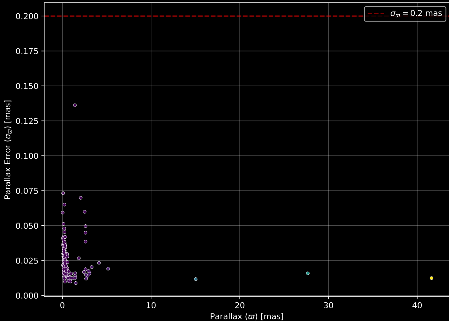
APOGEE DR17 Field: [113+04] Parallax Quality (n= 156)
