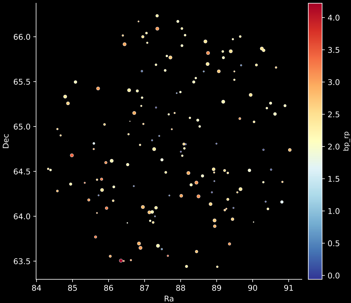
APOGEE DR17 Field: [113+04] Stars: 156
