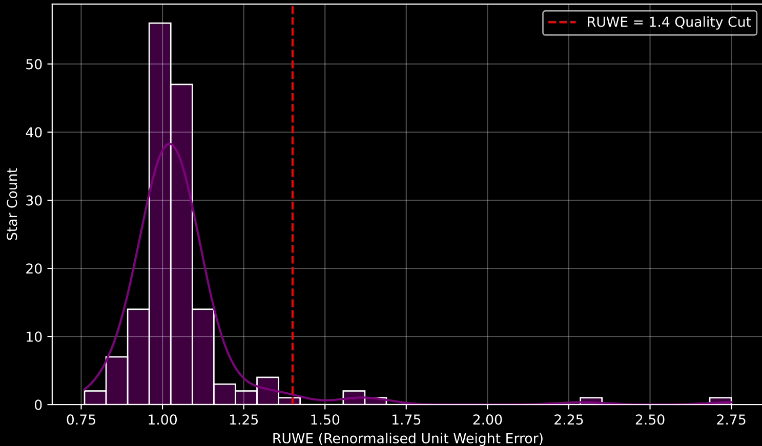
GAPOGEE DR17 Field [113+04] RUWE Distribution (n= 155)
