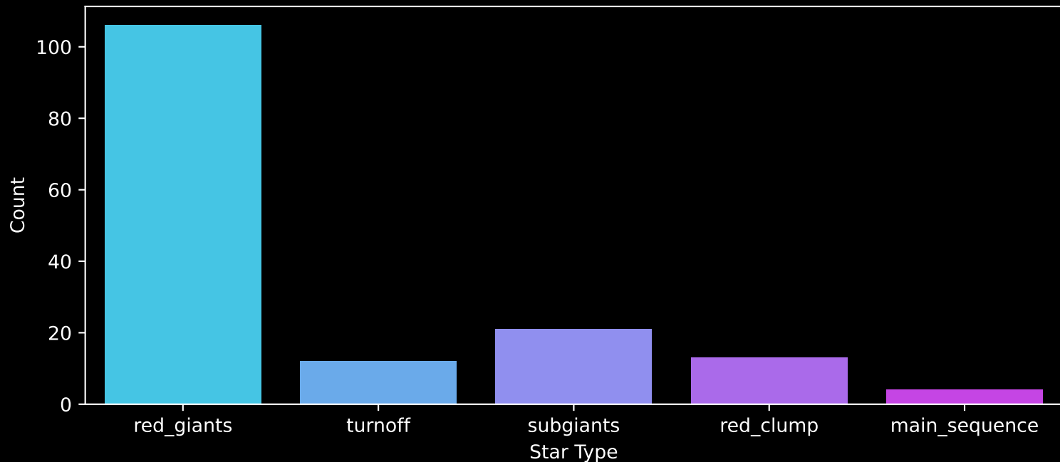
APOGEE DR17 Field: [113+04] Count plot of Star Type
