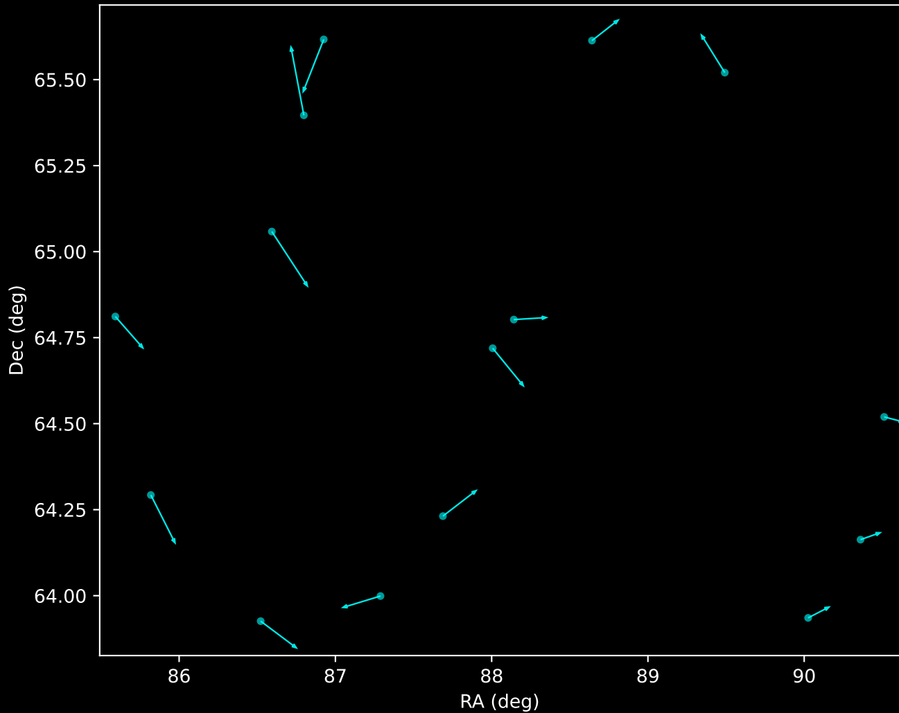
APOGEE DR17 Noise Stream Proper Motion Vectors (n=15)
