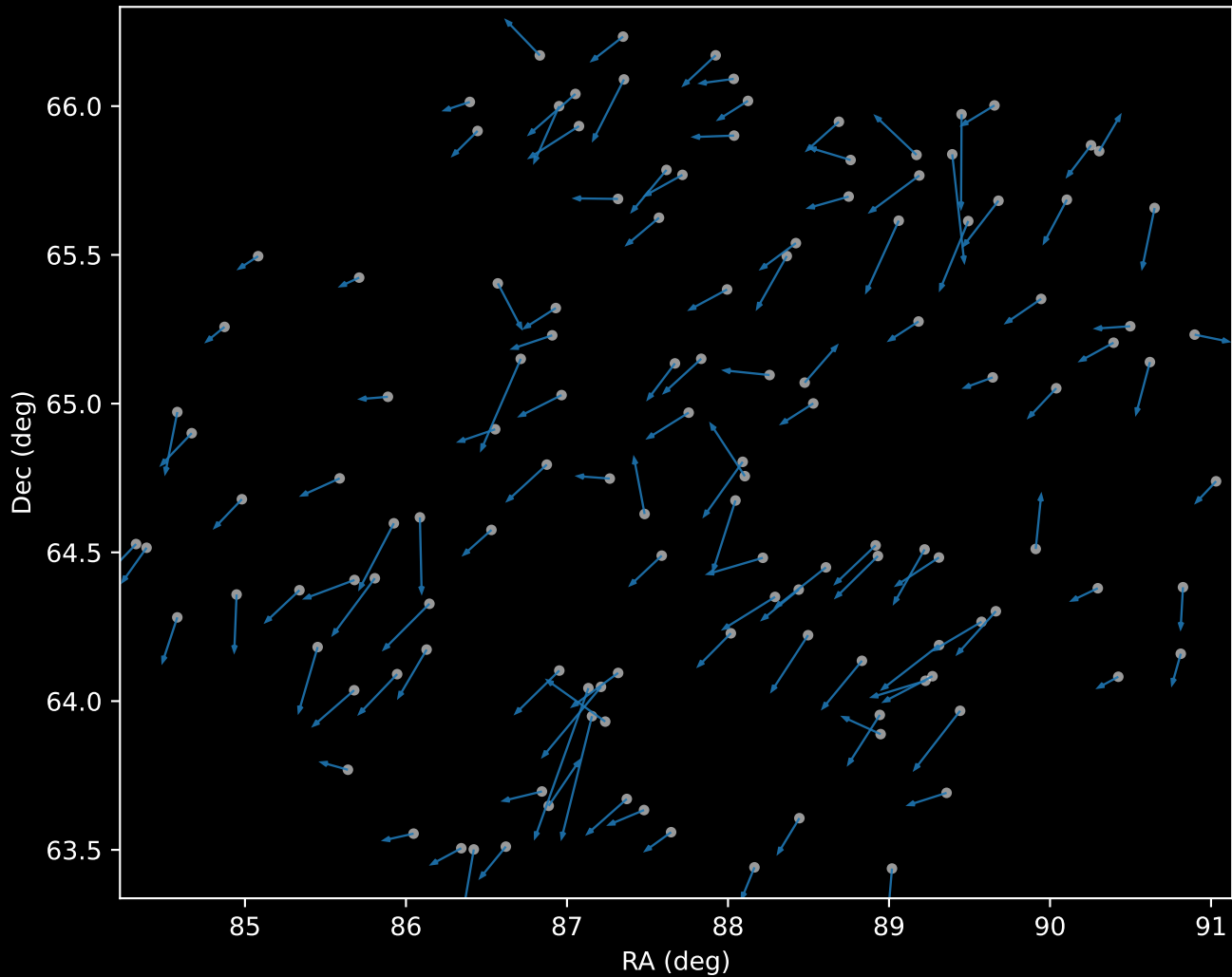
APOGEE DR17 Cluster 0 Proper Motion Vectors (n=129)
